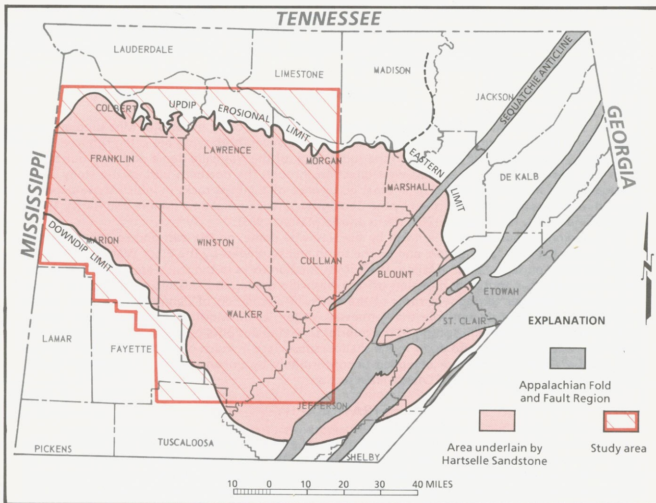
Figure 1.--Areal extent of the Hartselle Sandstone and outline of the study area.
